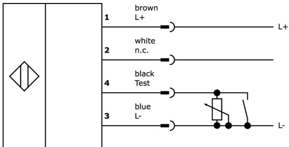
Test input: Transmitter off = 0V Transmitting power adjustable via 10KΩ potentiometer
