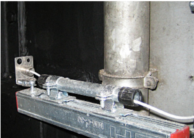
ipf_FHW_Neukoelln004 and ipf_FHW_Neukoelln005: Close-up of the measuring head, which was fastened to an aluminum profile in the front area and can be used in ambient temperatures of up to +180°C without cooling.
