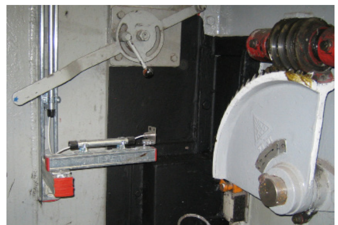
ipf_FHW_Neukoelln007: Because different temperatures occur on each side of the feed hopper, an infrared sensor was installed on each side of the hopper (at left here) for monitoring.
