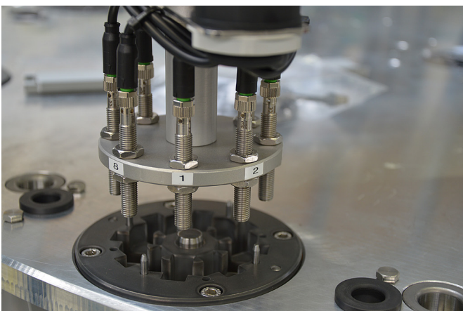
The receptacle for the rotor, to which the eight magnets are mounted with alternating polarity. With the final placing and pressing an iron packet, the insert element for the plastic housing is completed.
