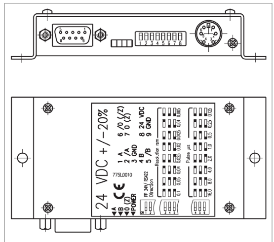
Abb. 1: Montage / Anschlüsse
