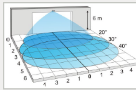
Mounting height: 6 m Boost function: ON Factory values
