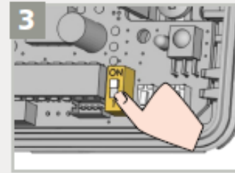
If mounting height > 4.5 m, activate BOOST function by DIP-switch.
