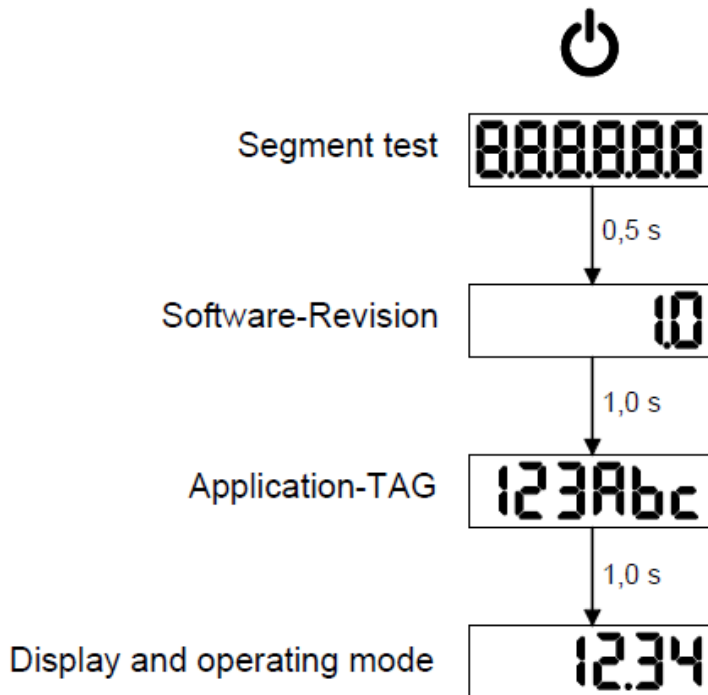
Figure 11: Power-up procedure
