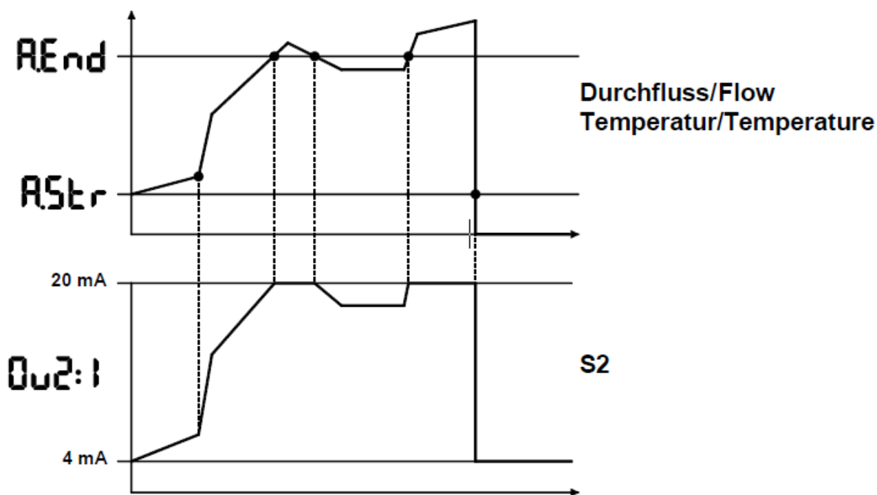
Figure 4: operating mode analog output
