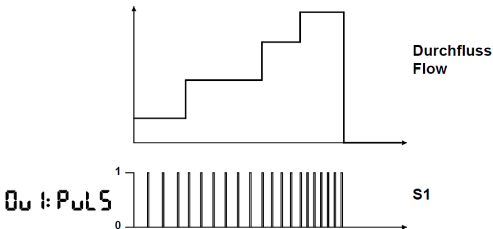
Figure 3: Operating mode pulsating output
