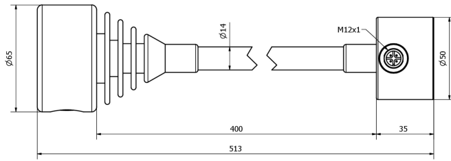
Dimensional drawing AO000318
