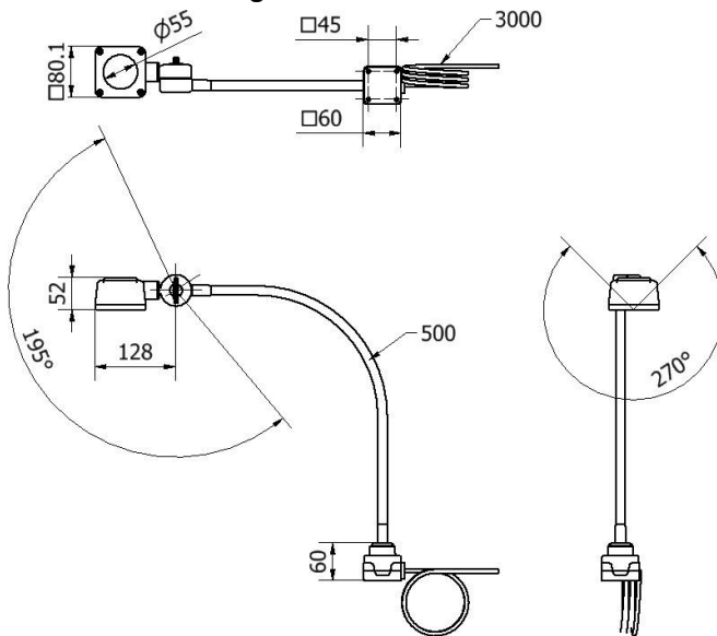
Dimensional drawing EB800120
