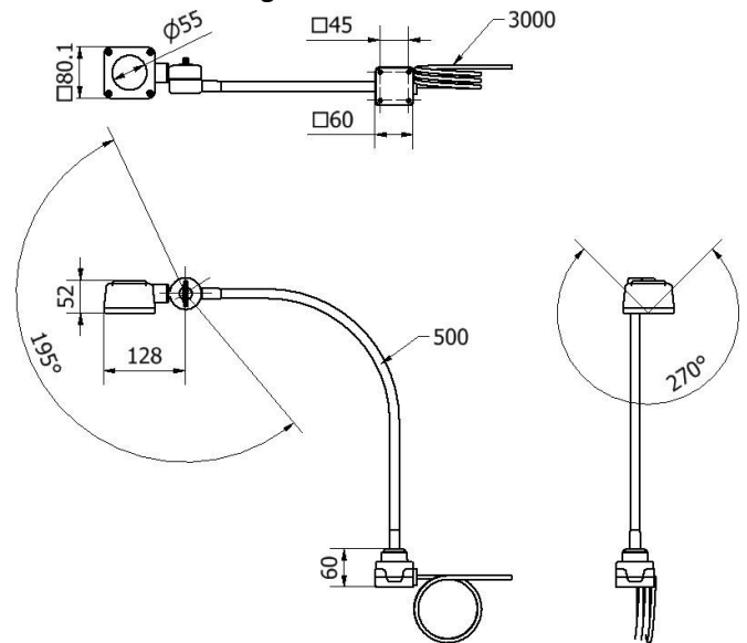
Dimensional drawing EB804140
