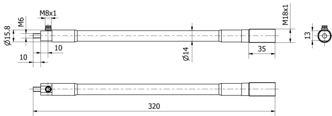
Dimensional drawing EB180170
