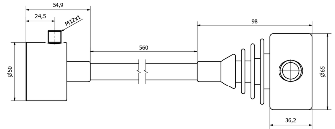
Dimensional drawing AO000397
