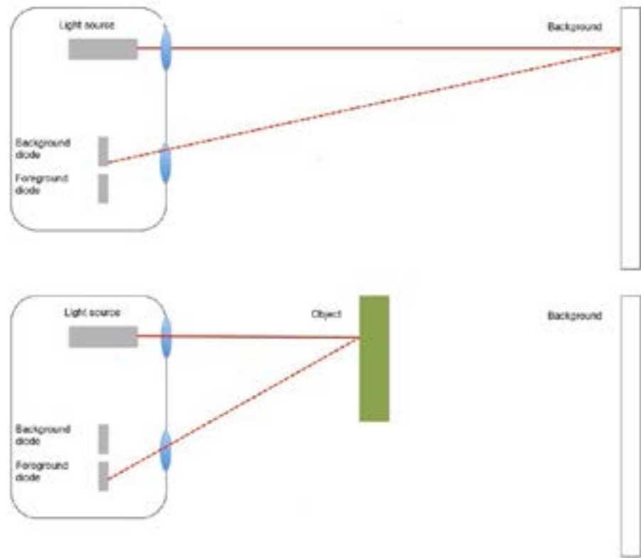
Operating principle of mechanical background suppression.
