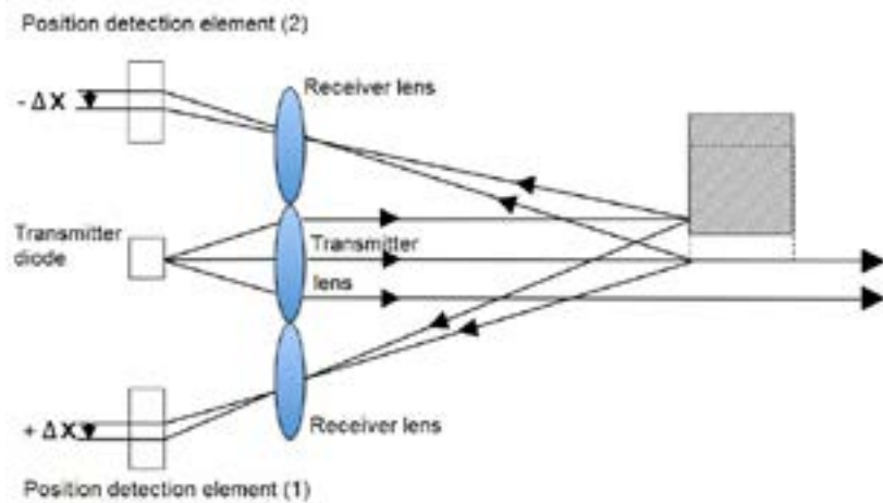
Operating principle of background suppression according to the three-beam.
