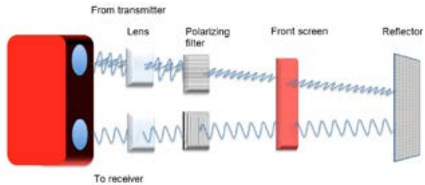
Operating principle of a polarizing filter. The filter of the transmitting optics is only permeable for a certain oscillation axis of the light. The same also applies to the filter at the receiver end.
