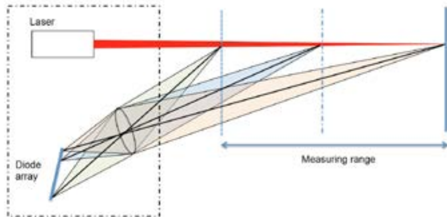
Operating principle of background suppression with a diode array.
