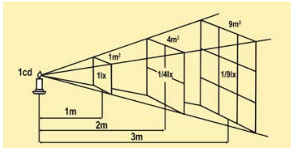
The photometric distance law states that illuminance decreases by the square of the light source.
