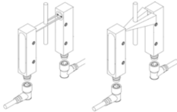
Laser light barrier on left; conventional light barrier on right.
