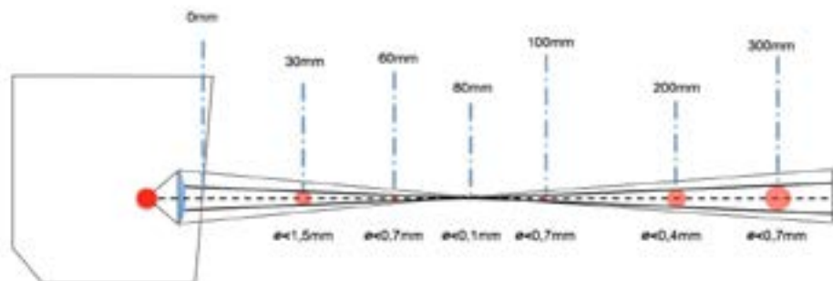
The smallest objects can be detected at the focus of the laser beam. The positioning and repeat accuracy is also greatest at this point.
