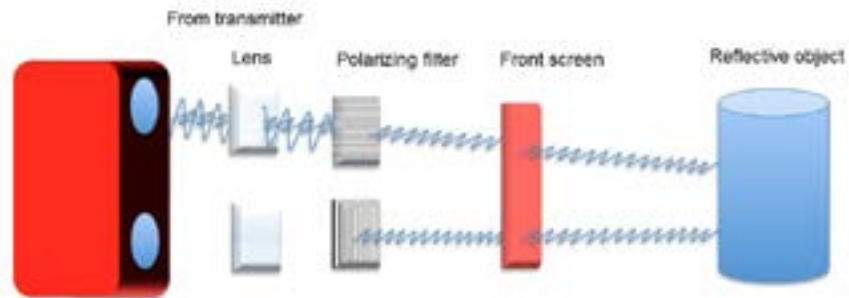
The light reflected by the object cannot pass through the polarizing filter; the object is therefore not reliably detected.
